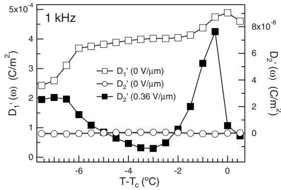
FIG. 1. Temperature dependences of the real parts of D_1(\omega) and D_2(\omega) measured simultaneously on cooling process at the frequency of 1 kHz. T_c indicates the transition point from the Sm-A phase to Sm- C_\alpha^* phase as decreasing the temperature.
