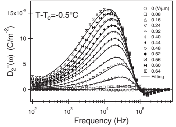
FIG. 4. Dependence of the imaginary part of D_2''(\omega) on dc field at T - T_c = -0.5 °C ( \text{Sm-C}_\alpha^* ).
