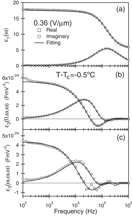
FIG. 3. Typical frequency dispersions of (a) \epsilon_1(\omega) , (b) \epsilon_3(0, \omega, \omega) , and (c) \epsilon_3(\omega, \omega, \omega) obtained at T - T_c = -0.5 °C in the \text{Sm-C}_\alpha^* phase at a dc field of 0.36 \text{V}/\mu\text{m} .
