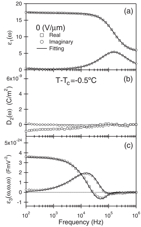
FIG. 2. Typical frequency dispersions of (a) \epsilon_1(\omega) , (b) D_2(\omega) , and (c) \epsilon_3(\omega, \omega, \omega) obtained at T-T_c = -0.5^\circ\text{C} in the Sm- C_\alpha^* phase at zero dc field.
