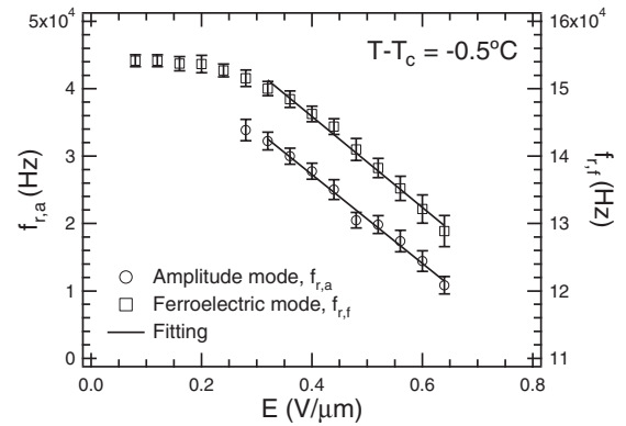
FIG. 5. Dc field dependences of the relaxation frequencies obtained from the linear and the second-order nonlinear dielectric spectroscopies. f_{r,f} and f_{r,a} are the relaxation frequencies of the ferroelectric mode obtained from the fitting result using Eq. (9) and the amplitude mode using Eq. (8), respectively.
